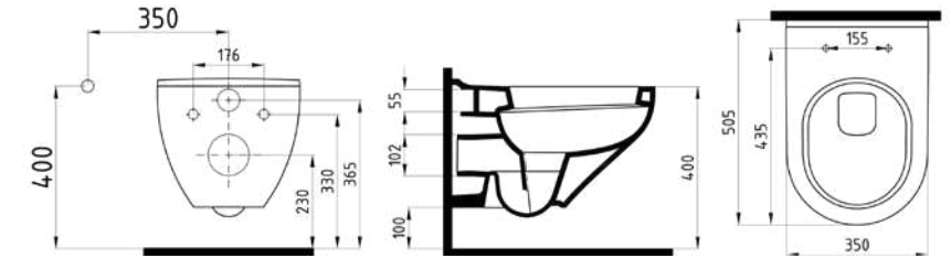
ASMA KLOZET IOKA050AMVP1W5000 500x350 mm
