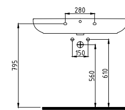
DUVAR MONTAJLI LAVABO BATARYA DELİKLİ / TAŞMA DELİKLİ MDLS09001FD1W5000 900x420 mm
