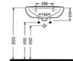
BEDENSEL ENGELLİLER İÇİN LAVABO TPLE06001VD1W3000 600x510 mm
